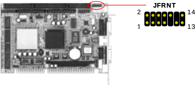
Connector: JFRNT (CN4) Type: onboard 14-pin header
